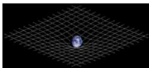
Figura 1: Wikipedia 2012 - General relativity (Spacetime curvature)
